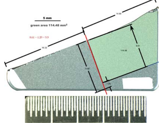
Figure 5 Cutting plan for 60000 DOS. The toe and heel clip marks (shown in white) were transposed from the SW side to verify location of scribe lines.
