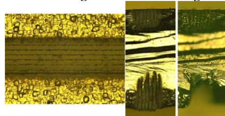
Figure 3 Channel created by SCSCS (left image-plan view) and (right image on-end view) before and after cleaning. Shown is a non-flight sample.
