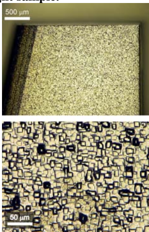
Figure 2. Crystallographic orientation of FZ-Si used for placement of scribe lines. Shown is a non-flight sample.
